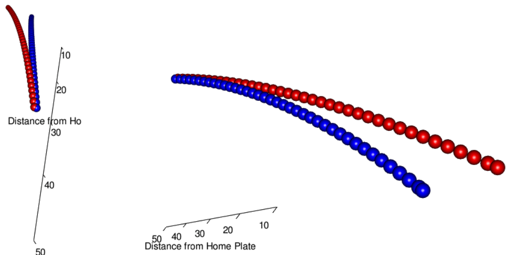
Figure 8: 3D scatterplot of pitches from Rivera. Pitches are plotted every one-hundredth of a second. Cutting fastballs are shown in red and four-seam fastballs are shown in blue. The left hand plot takes a viewpoint of Rivera and the right hand plot takes a viewpoint near the umpire. Note these are static pictures of an interactive object.
